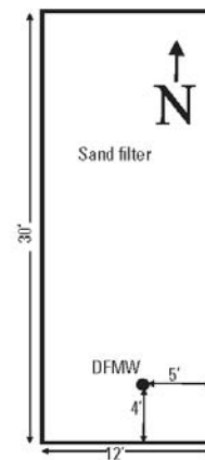
Drainfield Monitoring Well (DFMW) 434741121273101 Sand filter
