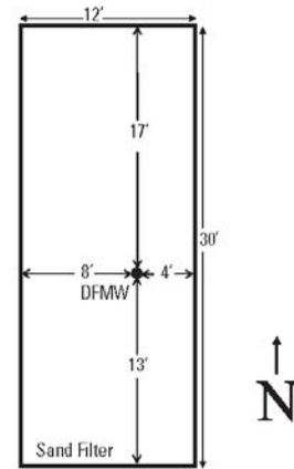
Drainfield Monitoring Well (DFMW) 434347121293901 Sand filter
