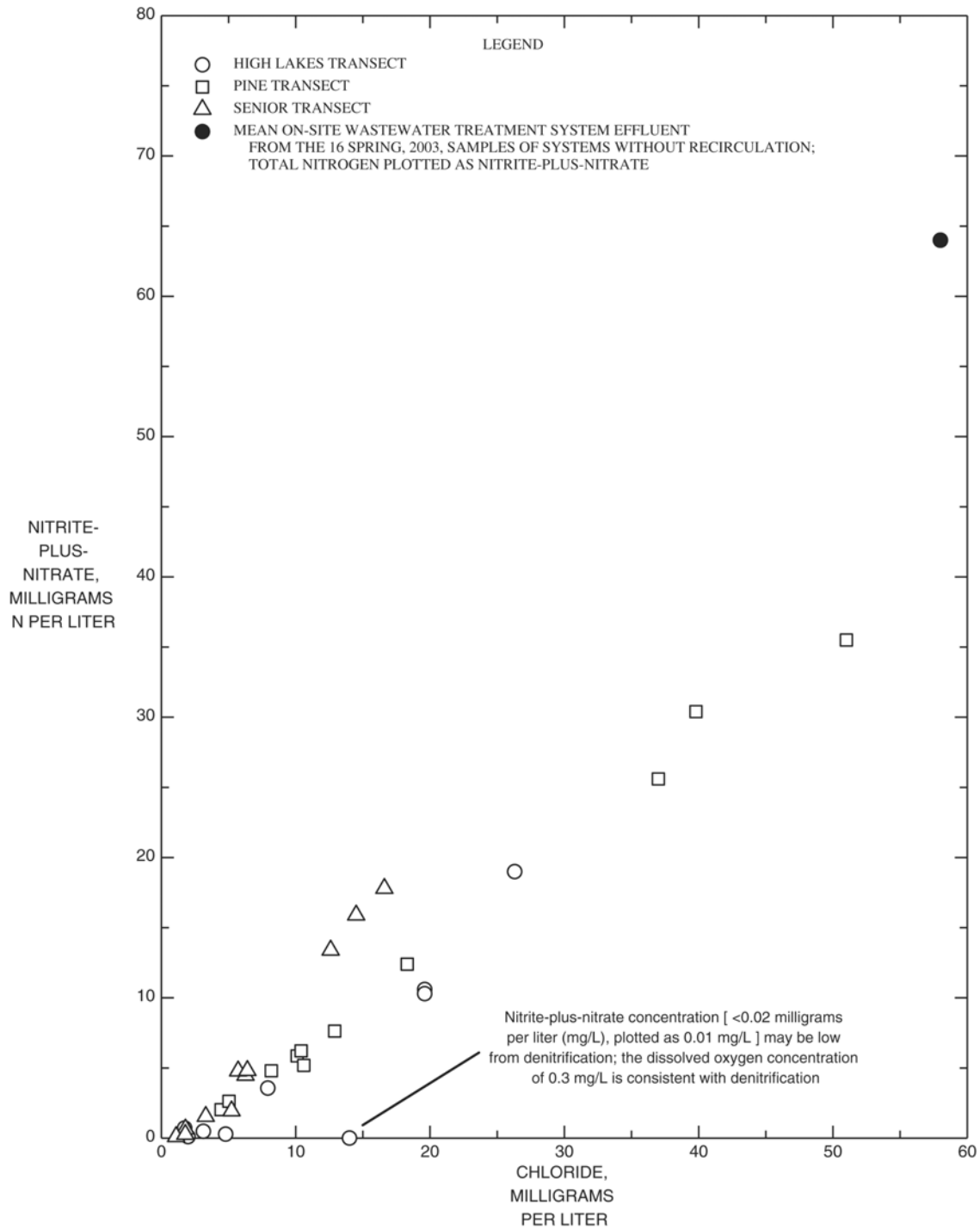
Figure 3-1: Relation Between Chloride and Nitrite-Plus-Nitrate Concentrations for the Three Transects Near La Pine, OR
