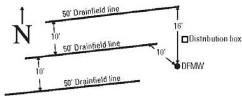
Drainfield Monitoring Well (DFMW) 434236121310501 Septic tank with gravity-feed drainfield lines
